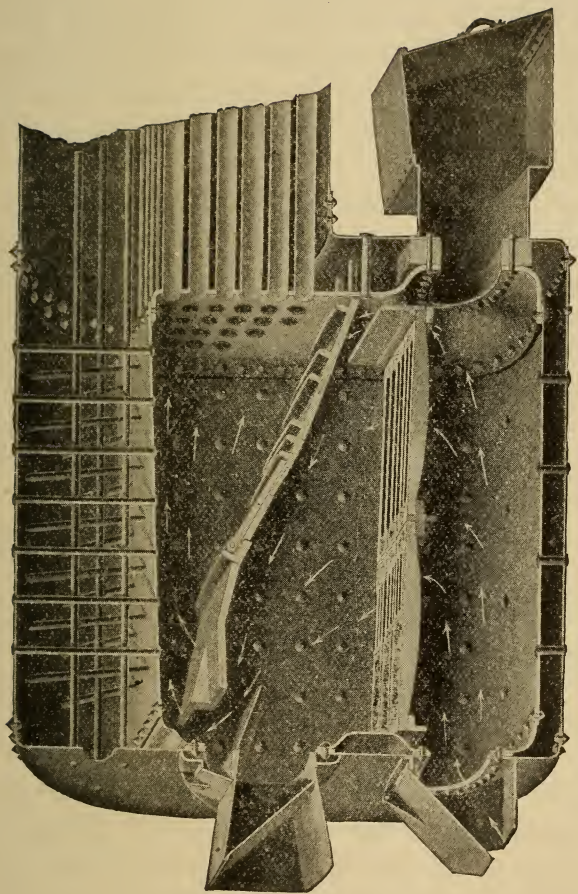
FIG. 22.—FIRE-BOX OF THE PORT HURON STRAW-BURNING BOILER.
